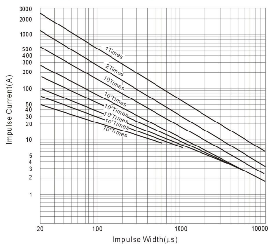
Surge Life Time Reting [820LD10 to 112KD10]
